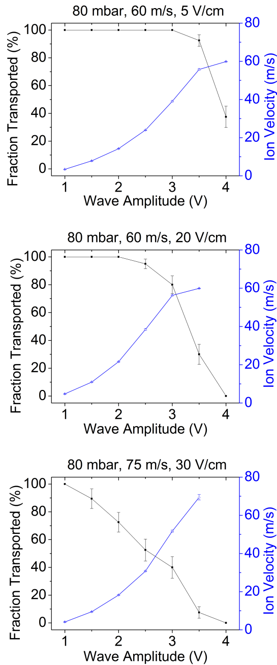
Figure 6.10: Surf2D ion transport efficiency results over 10 cm (black squares) and velocity results (blue triangles) as a function of wave amplitude. Experimental conditions are simulated as indicated, and the approximate maximum ion velocity can be determined for a given efficiency. Common parameters: a = 0.375 mm, \gamma = 0.67 , 8.47 MHz and 65 V. The wave amplitudes for the experimental results are shown in Figure 6.8.
