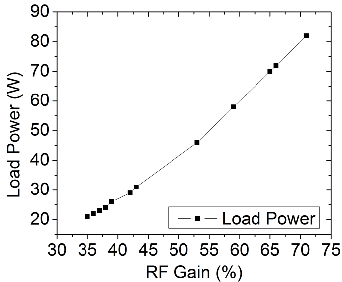
Figure 4.7: Above: The RF pickup (closed circles) and amplitude (open squares) at the chamber feedthroughs increase roughly linearly as the gain of the RF generator also increases. Below: The power delivered to the carpet and circuit increases nonlinearly with RF amplifier gain at low values of gain.
