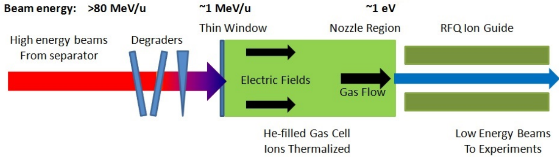
Figure 1.2: Schematic of the beam thermalization process. Most of the ions' kinetic energy is removed by the degraders before the ions pass into the gas cell. The ions are thermalized by the helium buffer gas and directed to the nozzle extraction region by electric fields [1]. For interpretation of the references to color in this and all other figures, the reader is referred to the electronic version of this dissertation.
