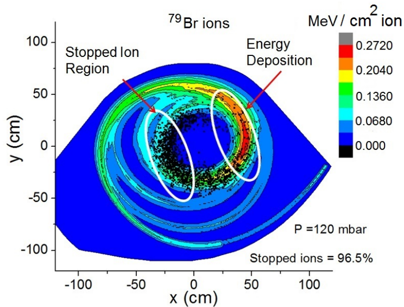
Figure 1.3: (Left) Schematic of the cross section of the cyclotron gas stopper. The blue lines designate the beam envelope of the first turn of the incoming ^{79}\text{Br} ions [7]. (Right) Simulated stopping region and energy deposition of ^{79}\text{Br} in 120 mbar of helium gas. A high stopping efficiency (96.5%) is achieved [7] in the simulation.
