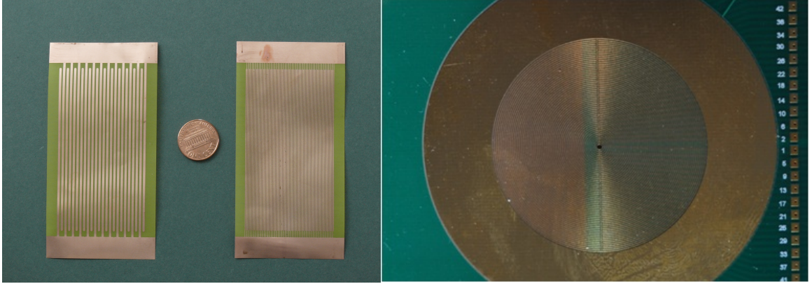
Figure 2.3: Examples of the two RF carpet electrode geometries. Left: RF carpets with linear electrodes (and two different pitches) used by Pang [10]. The pitch, a , is the sum of one electrode and one gap width. Right: RF carpet with concentric electrodes developed and employed by Wada [3].
