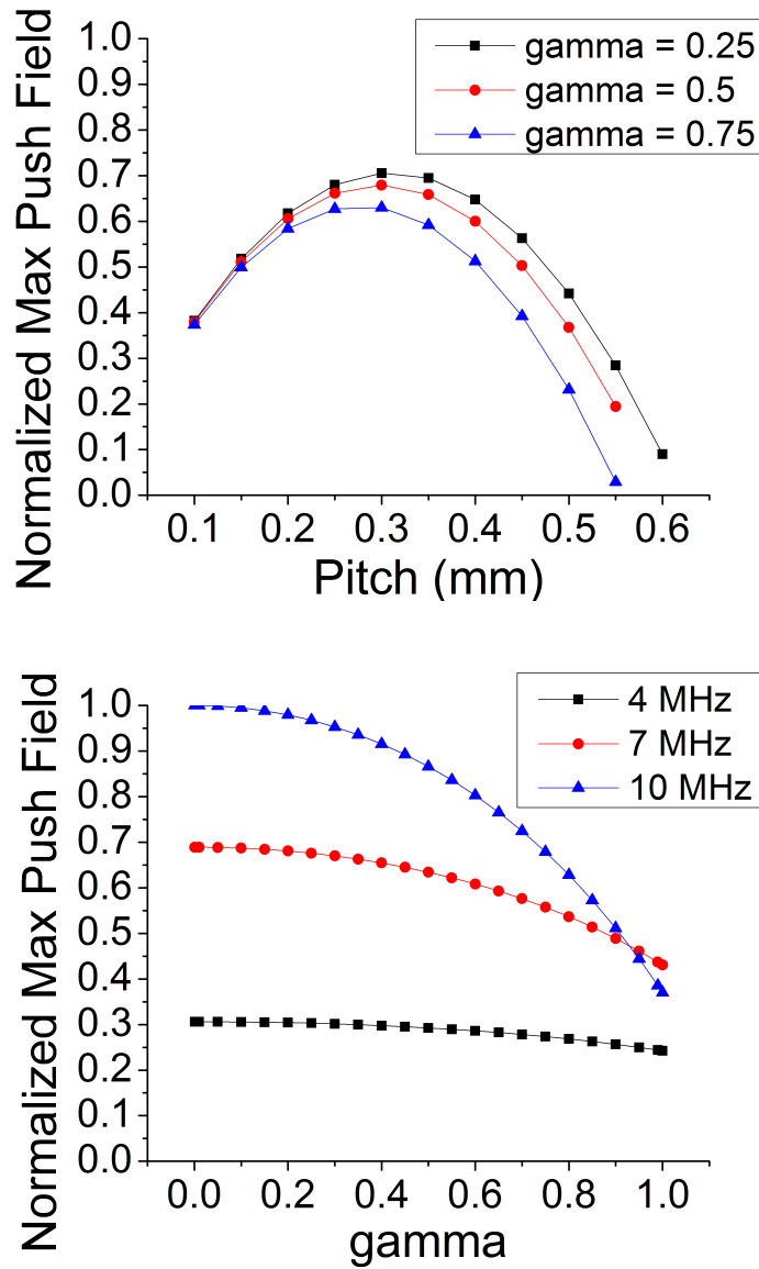
Figure 2.7: Comparison of the repelling force on a 23 u singly-charged ion for various values of carpet pitch, \gamma , and RF frequency. The maximum push field in Equation 2.1.2.1 is used as a measure of the repelling force. The units have been normalized to the value for pitch = 0.375 mm, \gamma = 0.001 at 10 MHz. A helium gas pressure of 100 mbar, temperature of 295 K, and a RF amplitude of 75 V were used in the calculations. Above: The effect of varying \gamma increases with the RF carpet pitch. A RF frequency of 7 MHz was chosen for this calculation due to 7 MHz being the approximate maximum repelling frequency for a = 0.5 mm (see Figure 2.5). Below: Varying \gamma is shown to effect the maximum repelling force significantly at high ( \sim 10 MHz) RF frequencies. For this calculation, a = 0.375 mm.
