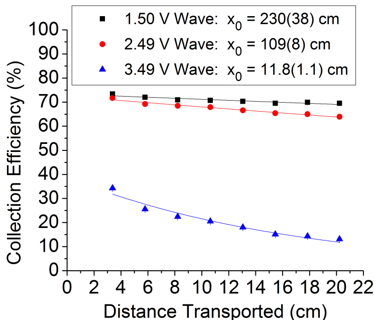
Figure 6.5: Collection efficiency as a function of the distance traveled by K^+ ions at three different wave amplitudes. The solid lines represent the best fit of Equation 5.1.1.1 to the data, and the half distances, x_0 , are listed on the graph. Parameters: a = 0.375 mm, \omega = 0.67 , 80 mbar, 20 V/cm push field, 8.47 MHz RF frequency, 65 V RF amplitude, and 60 m/s wave velocity.
