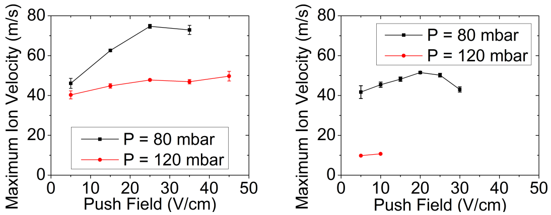
Figure 5.13: Maximum ion transport velocities with a half distance greater than 0.5 m as a function of push field. Left: Experimental results of Rb + ions at buffer gas pressures of 80 and 120 mbar. Right: Experimental results of K + ions at the same buffer gas pressures [12].
