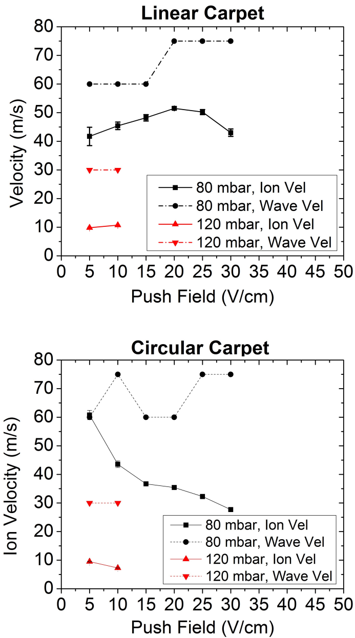
Figure 6.11: Comparison of the maximum ion velocities obtainable with a half distance greater than 0.5 m. Above: Best results for K^+ ions (see Figure 5.12). Below: The analogous semi-circular prototype results (see Figure 6.9.)
