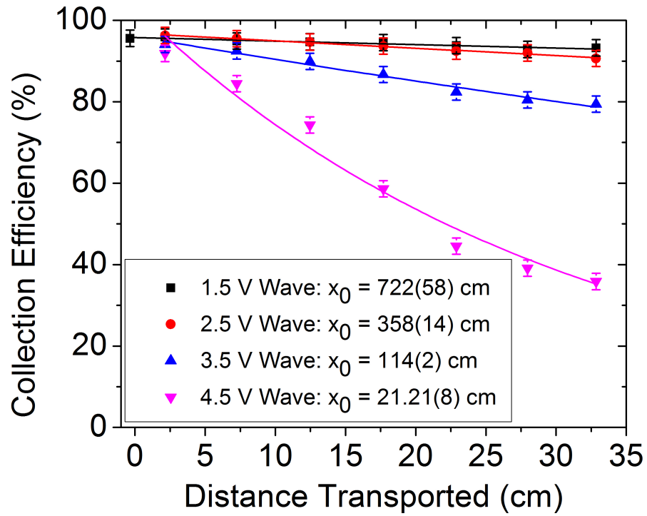
Figure 5.9: Collection efficiency as a function of the distance traveled by K^+ ions at four different wave amplitudes. The solid lines represent the best fit of Equation 5.1.1.1 to the data, and the half distances, x_0 , are listed on the graph. Parameters: a = 0.375 mm, \gamma = 0.67 , 80 mbar, 20 V/cm Push, 6.8 MHz RF frequency, 75 V RF amplitude, 60 m/s wave velocity [12].
