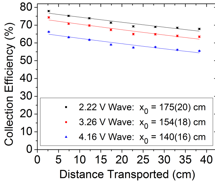
Figure 5.5: Collection efficiency as a function of the distance traveled by \text{Rb}^+ ions at three different wave amplitudes. The solid lines represent the best fit of Equation 5.1.1.1 to the data, and the half distances, x_0 , are listed on the graph. Parameters: a = 0.375 mm, \gamma = 0.67 , 120 mbar, 45 V/cm push field, 6.69 MHz RF frequency, 66 V RF amplitude, and 60 m/s wave velocity.
