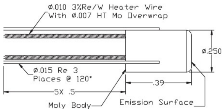
Model 101139 Ø.250" Ion Source
