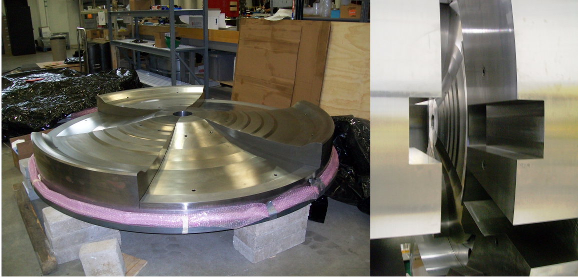
Figure 7.1: Left: Photograph of the six sector magnet pole steel during assembly. Right: Photograph of the pole steel inside the vertical magnet yoke of the cyclotron gas stopper.
