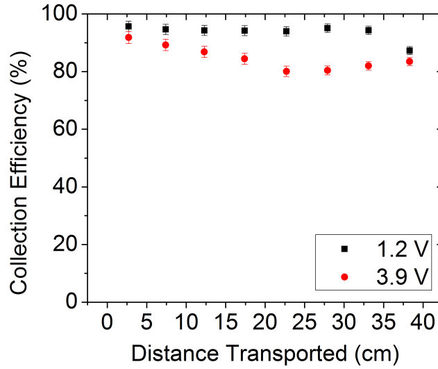
Figure 5.4: Collection efficiency as a function of transport distance for \text{Rb}^+ ions at two wave amplitudes with the linear prototype carpet. Parameters: a = 0.375 mm, \gamma = 0.67 , 120 mbar, 6.51 MHz RF frequency, 81 V RF amplitude, 12 V/cm push field and 15 m/s wave velocity.
